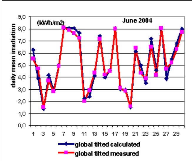
Fig. 1.21: Comparison of the daily solar irradiation processed from the Helioclim-2 database and the daily solar irradiation measured on site on the tilted plane for June 2004.
